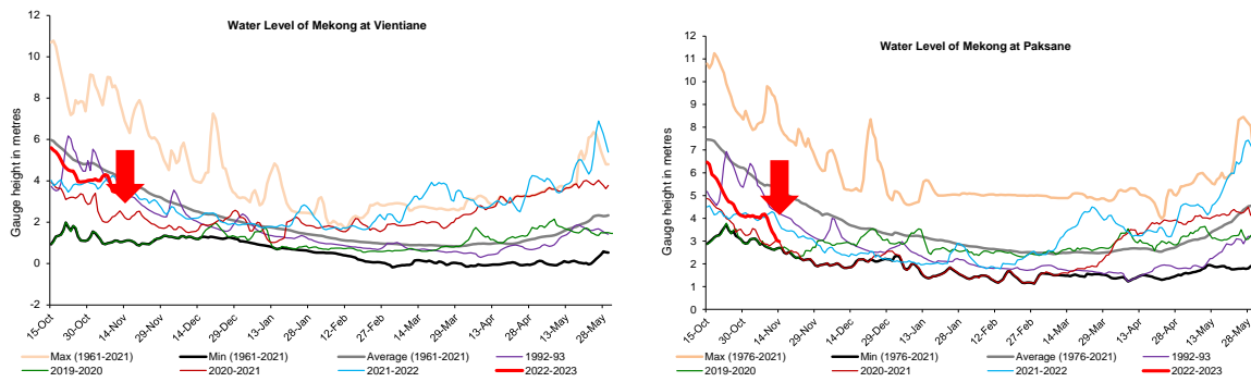
Figure 9. Water levels Veintaine and Paksane in Thailand and Lao PDR.
