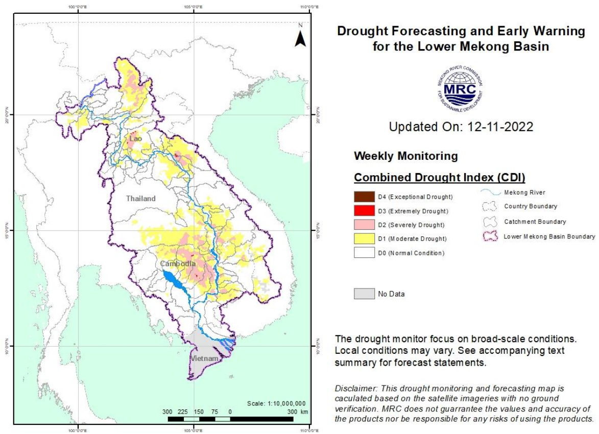
Figure 16: Weekly Combined Drought Index during November 6-12.
