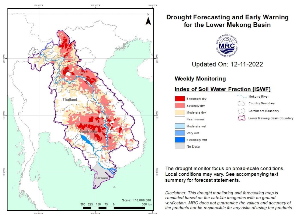
Figure 15: Weekly Index of Soil Water Fraction from November 6 to 12.
