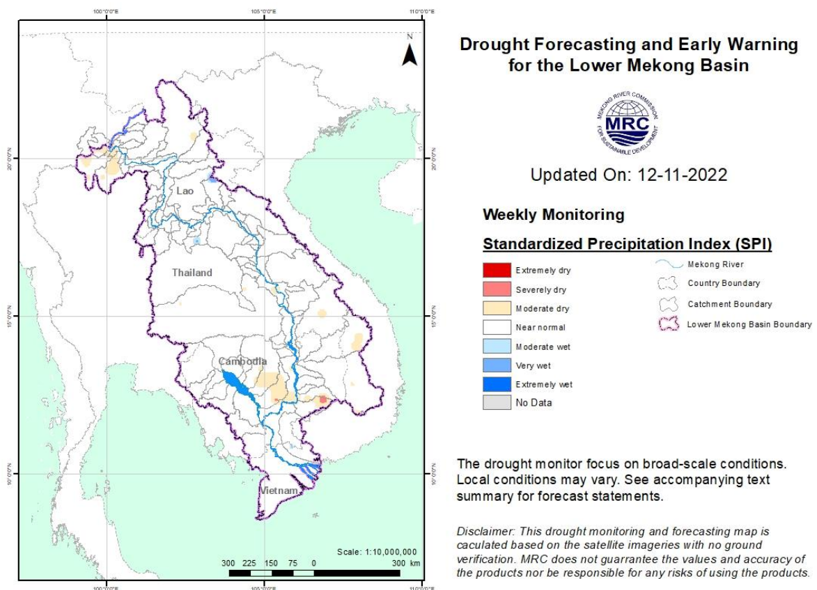
Figure 14: Weekly standardised precipitation index from November 6 to 12.
