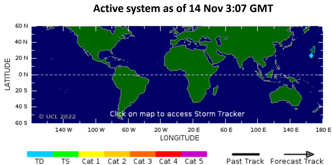
Figure 3: No tropical storm risk observed on 14 November 2022.
